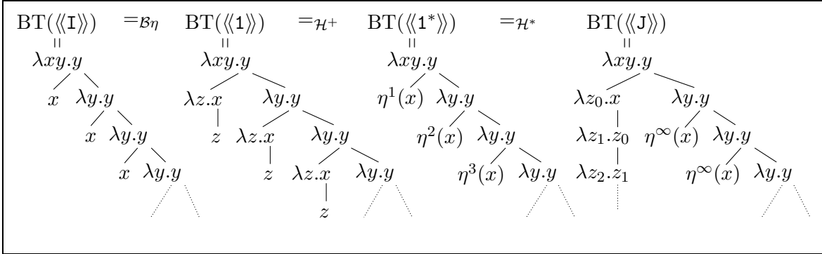
Figure 2: The Böhm trees of \langle\langle I \rangle\rangle , \langle\langle 1 \rangle\rangle , \langle\langle 1^* \rangle\rangle and \langle\langle J \rangle\rangle , where we set \eta^n(x) = \text{BT}(1^n x) and \eta^\infty(x) = \text{BT}(Jx) .
