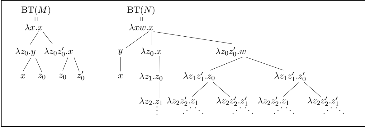
Figure 5: Two \lambda -terms M, N such that M \in \text{NF}_\beta , \mathcal{H}^* \vdash M = N , but \mathcal{H}^+ \vdash M \not\sqsubseteq N .
