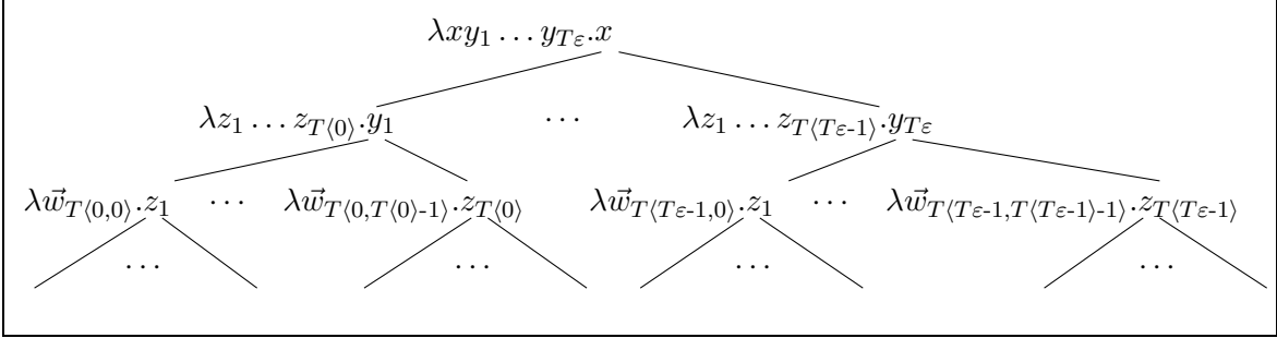
Figure 4: The Böhm-like tree of an infinite \eta -expansion of \mathbf{I} following T \in \mathbb{T}_{\text{rec}} . To lighten the notations we write T\sigma for T(\sigma) and \lambda\vec{w}_n for \lambda w_1 \dots w_n .
