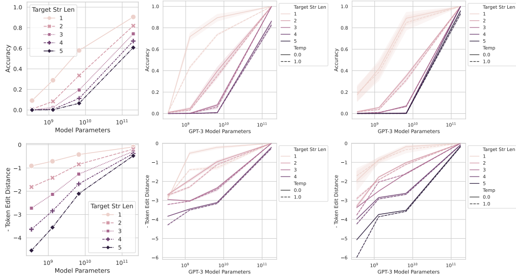
Figure 3: Claimed emergent abilities evaporate upon changing the metric. Left to Right: Mathematical Model, 2-Integer 2-Digit Multiplication Task, 2-Integer 4-Digit Addition Task. Top: When performance is measured by a nonlinear metric (e.g., Accuracy), the InstructGPT/GPT-3 [3, 24] family’s performance appears sharp and unpredictable on longer target lengths. Bottom: When performance is instead measured by a linear metric (e.g., Token Edit Distance), the family exhibits smooth, predictable performance improvements.
