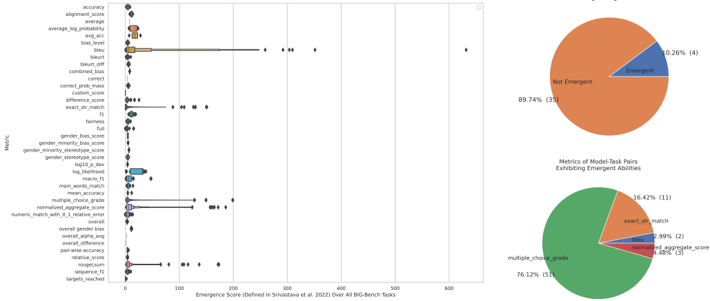
Figure 5: Emergent abilities appear only for specific metrics, not task-model families. (A) Possible emergent abilities appear with at most 5 out of 39 BIG-Bench metrics. (B) Hand-annotated data by [32] reveals emergent abilities appear only under 4 preferred metrics. (C) > 92% of emergent abilities appear under one of two metrics: Multiple Choice Grade and Exact String Match.
