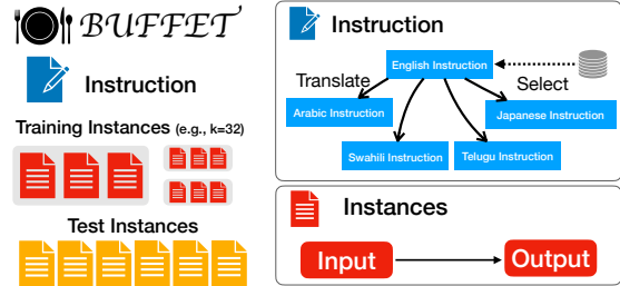
Figure 2: BUFFET includes 15 datasets, which are unified into the same single text-to-text format.
