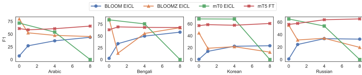
Figure 10: Effects of demonstrations on TYDIQA. The x -axis indicates the number of training instances used during the transfer.
