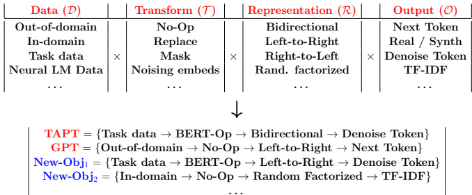
Figure 2: Our framework in the context of NLP. We decompose named objectives within our four staged taxonomy : \{\mathcal{D}, \mathcal{T}, \mathcal{R}, \mathcal{O}\} . By taking the cartesian product of choices across stages, we reproduce named objectives and discover new ones.
