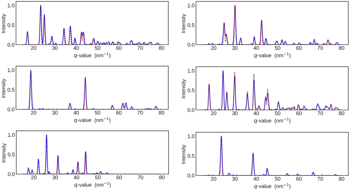
Figure 2. Al-Li-Fe basis patterns: Comparison between the six independent basis patterns as calculated by NMFk (blue solid line) and the end members used to generate the data (dotted red line). The maximum value in each pattern is normalized to 1.
