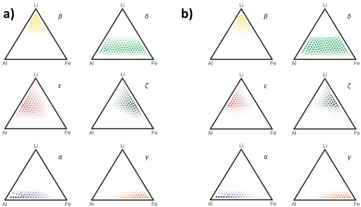
Figure 3. Phase weights for the Al-Li-Fe oxide data: The weights of each unique end member at a given composition. On the left (a) is the “ground truth” exact solution (from Ref. [11]), and on the right (b) are the weights as determined by NMFk method.
