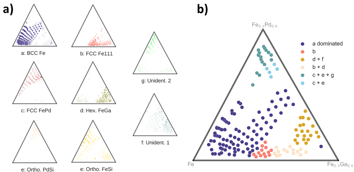
Figure 8. Structural phases and constructed phase diagram for the Fe-Ga-Pd data: a) The abundancies of the structures recovered by NMFk (noise excluded). b) Simplified phase diagram showing some of the major phases in the Fe-Ga-Pd phase diagram.
