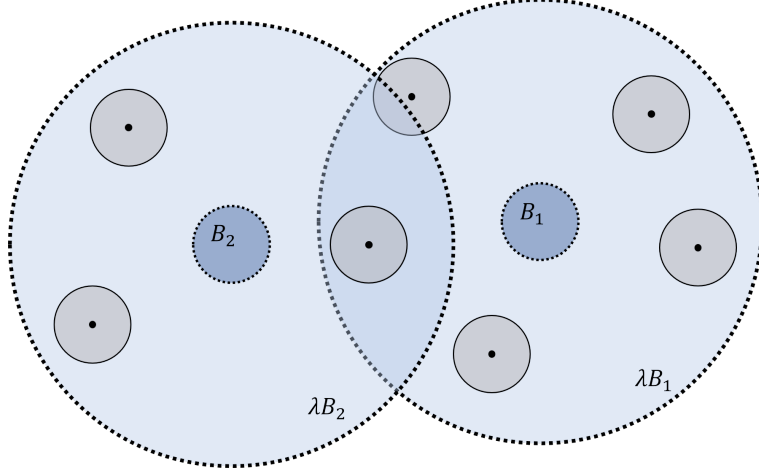
Figure 4: New heavy balls B_1, B_2 \in \mathcal{B}_{\mathcal{V}}^j are responsible for ejecting some of the previously heavy balls in \mathcal{B}_{\mathcal{U}}^j .
