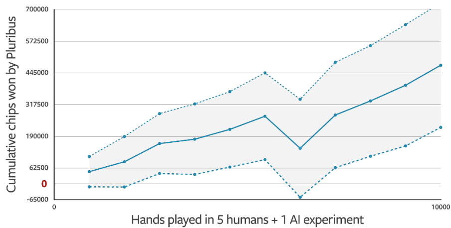
Fig. 5. Performance of Pluribus in the 5 humans + 1 AI experiment. Top: The lines show the win rate (solid line) plus or minus the standard error (dashed lines). Bottom: The lines show the cumulative number of chips won (solid line) plus or minus the standard error (dashed lines). The relatively steady performance of Pluribus over the course of the 10,000-hand experiment suggests the humans were unable to find exploitable weaknesses in the bot.
